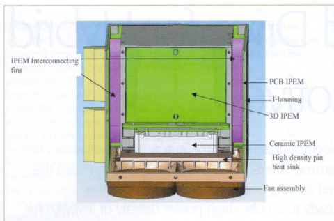
Figure 2: Complete assembly of the integrated drive converter
