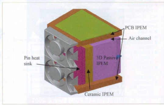
Figure 1: 3D layout of the integrated drive converter
