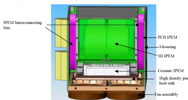
Figure 2 Complete assembly cross section
