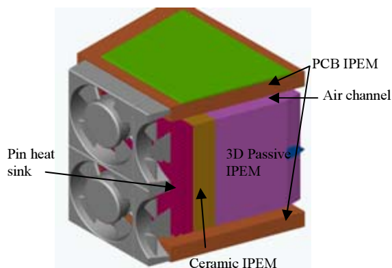
Figure 1: 3D layout of the system
