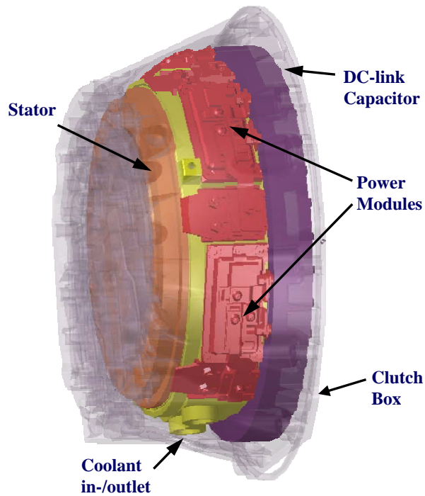
Fig. 2: X-ray view on the second generation inverter drive (50kW), integrated into the clutch-box of a passenger car.
