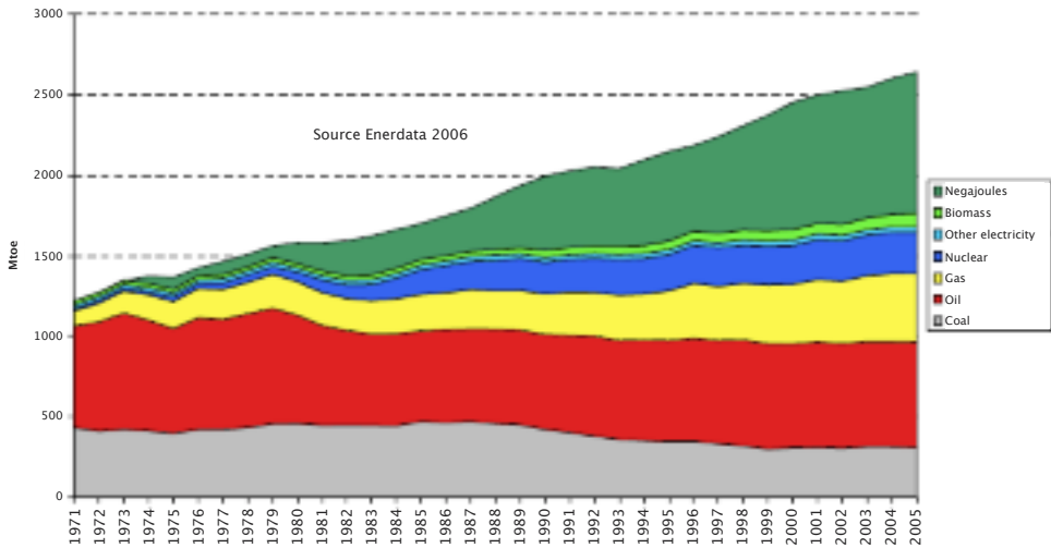
Figure 1: Negajoules have become the single most important energy resource (Source: [IEEP 06], p. 5).
