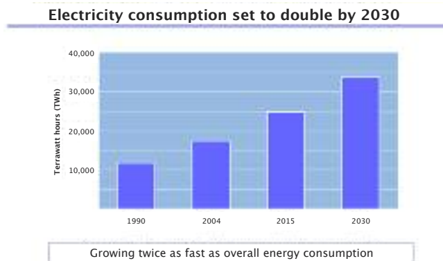
Figure 1: Electricity consumption forecast 1 (Source: International Energy Agency, IEA)
